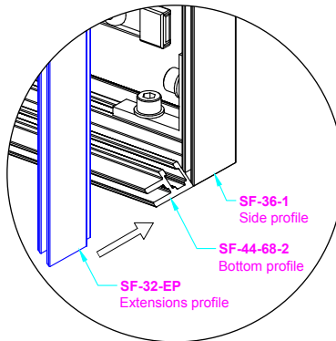
SF-32-EP Extensions profile
