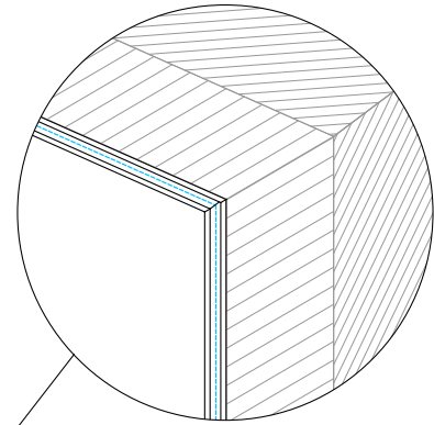
Frame in miter joint
